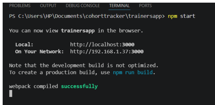
Figure 5: Terminal Output
